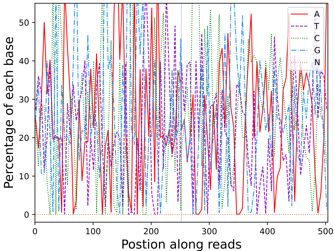
Base percentage along reads (R10314)
